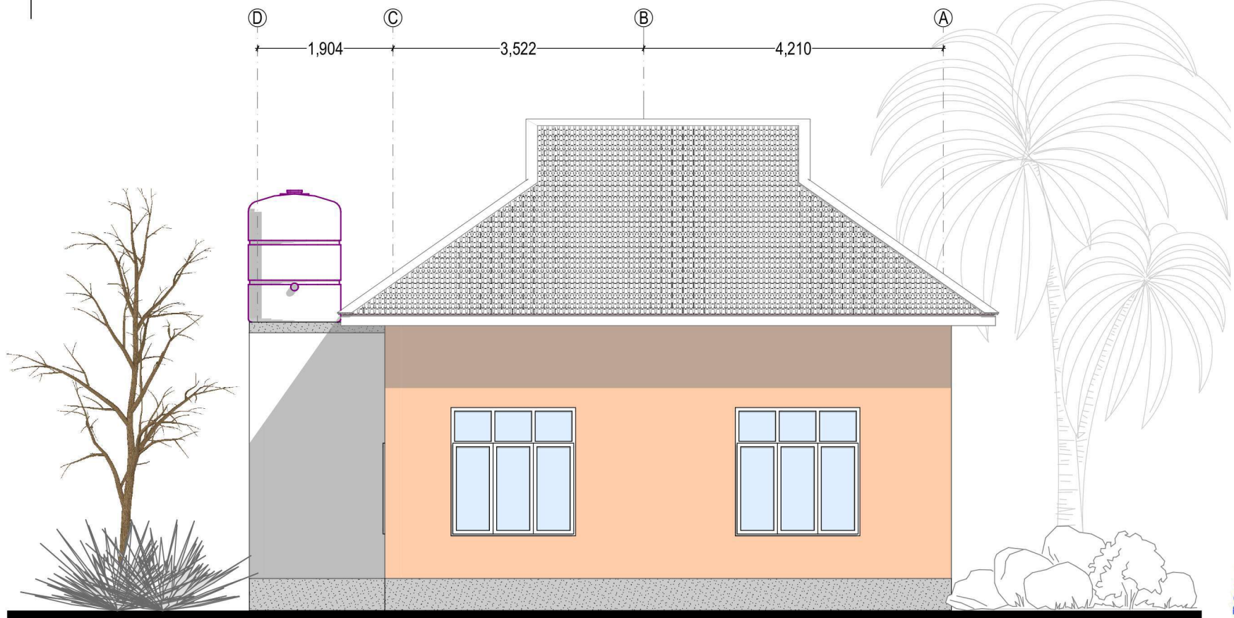
ELEVATION - 01 SCALE 1:75
