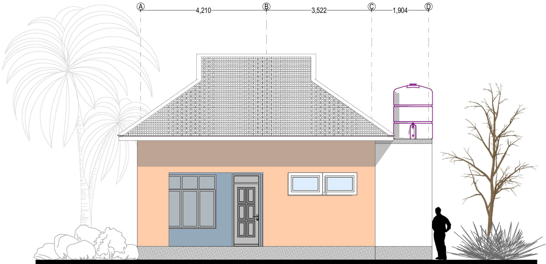
ELEVATION - 01 SCALE 1:75
