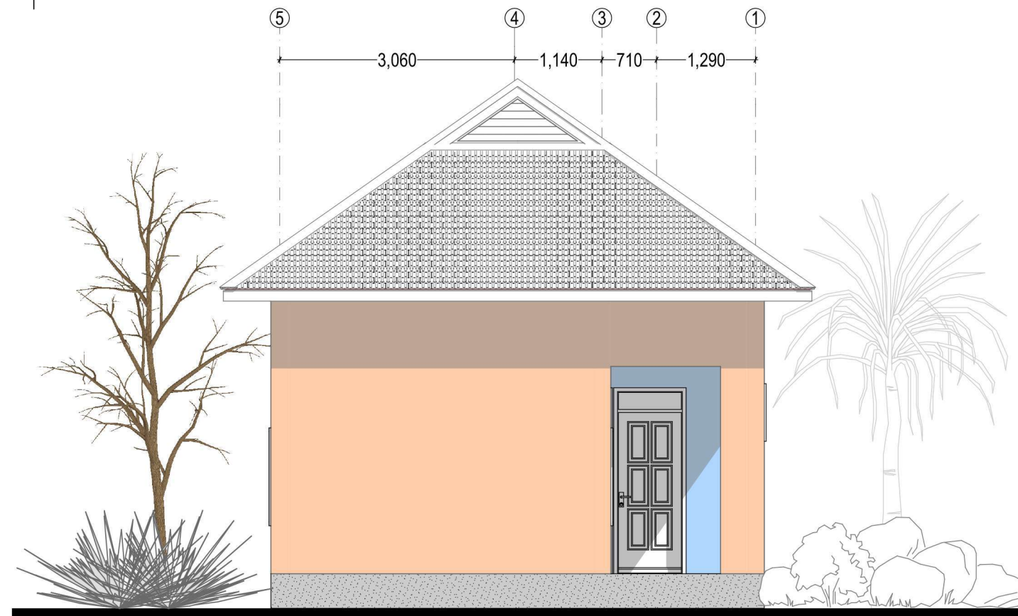
ELEVATION - 04 SCALE 1:70
