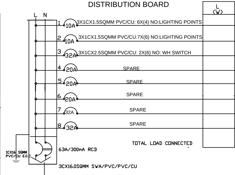
DISTRIBUTION BOARD
