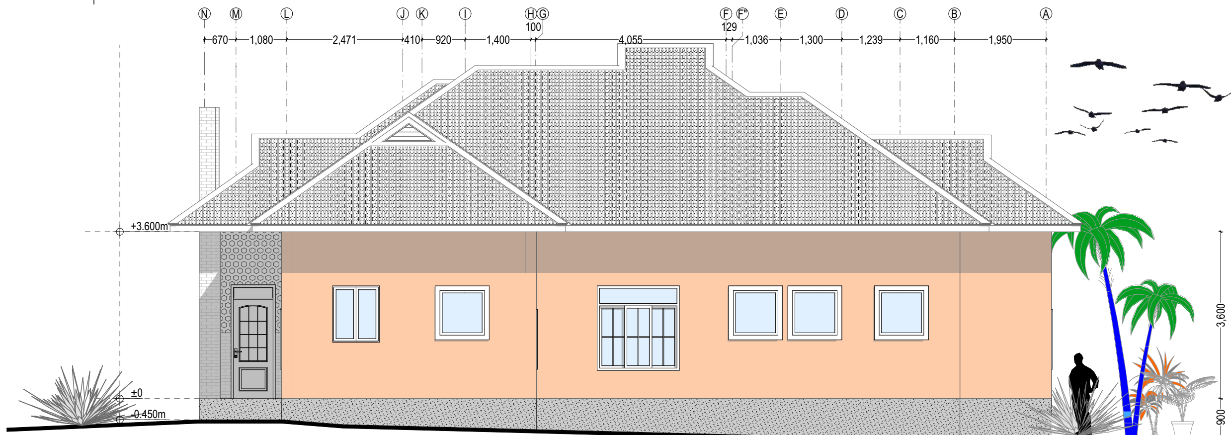
ELEVATION - 02 SCALE 1:80
