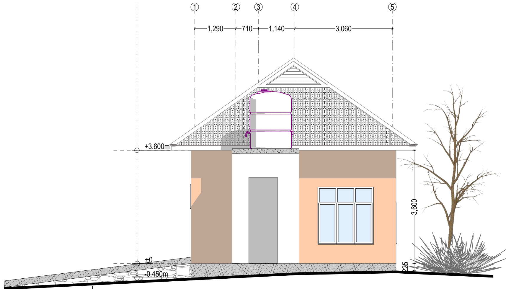
ELEVATION - 0 3 SCALE 1 : 7 0
