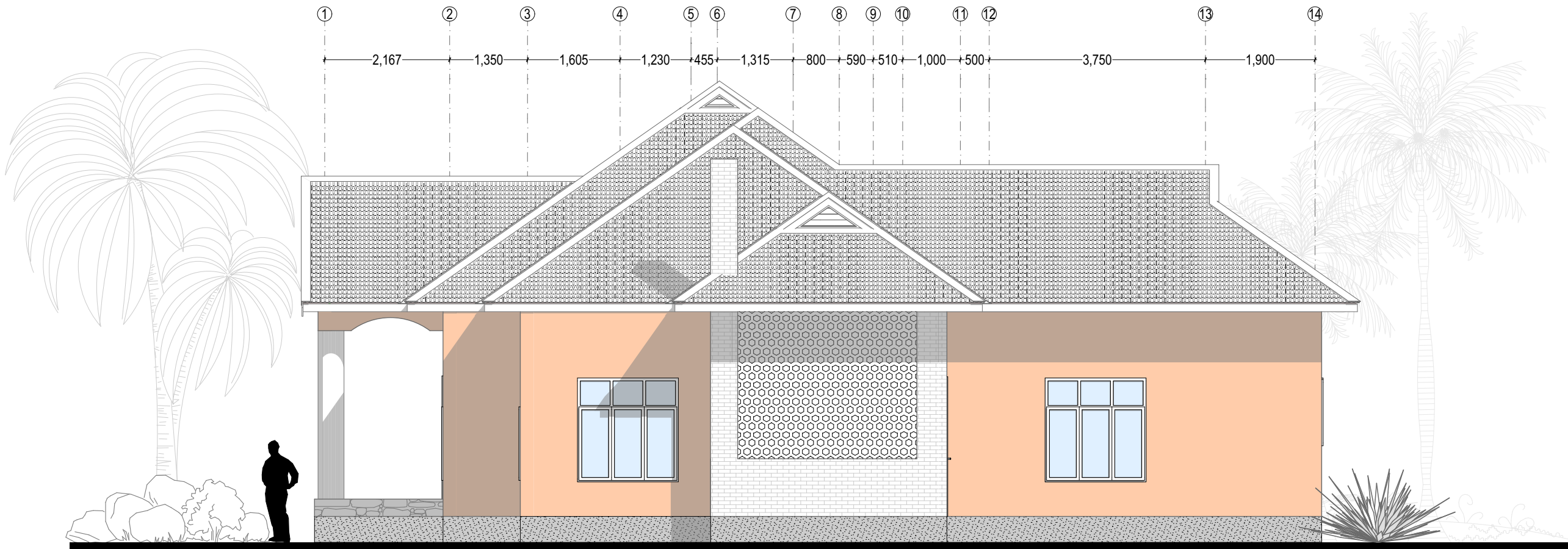
ELEVATION - 03 SCALE 1:80
