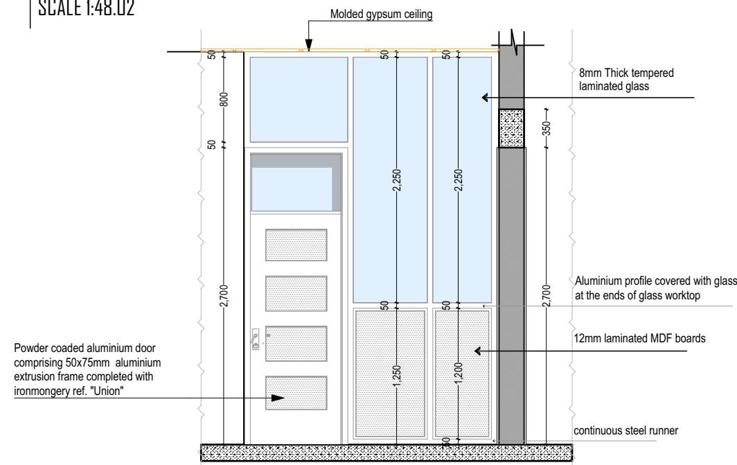
DRY WALL PARTITION DETAILED ELEVATION SCALE 1:48.02
