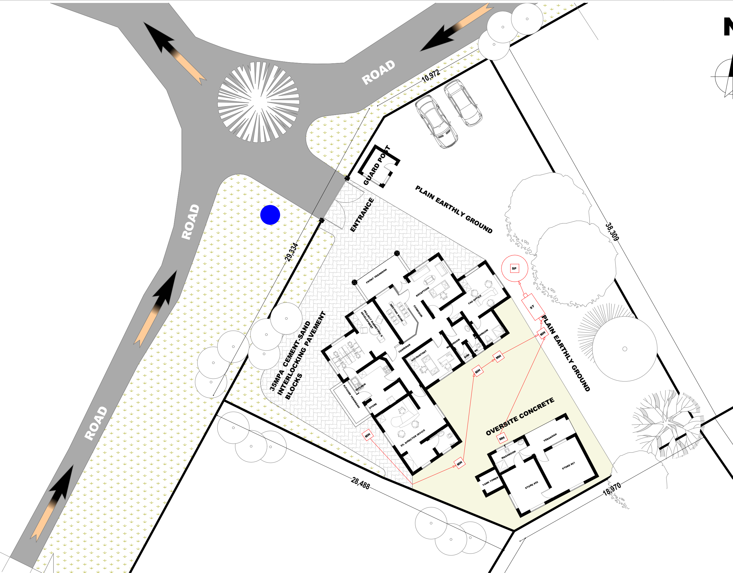
EXISTING SITE PLAN: PLOT No-157 & PLOT No-172 SCALE 1:200
