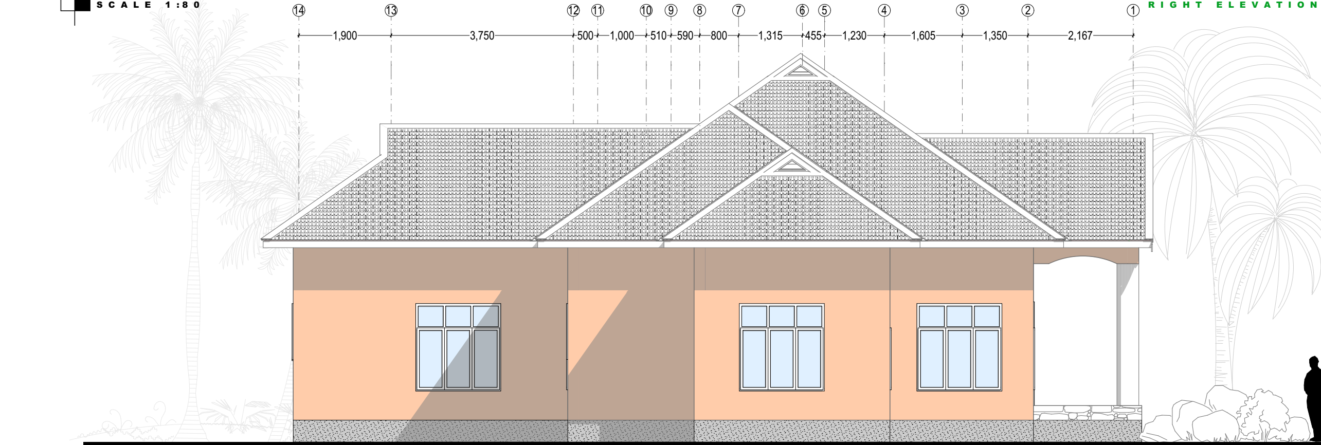
ELEVATION - 04 SCALE 1:80
