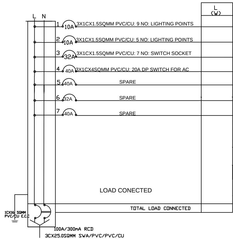
DISTRIBUTION BOARD
