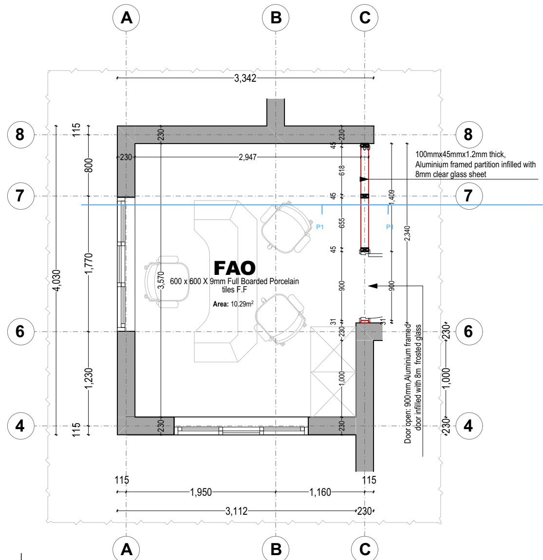
FAO OFFICE PARTPLAN + DRY WALL DETAIL SCALE 1:48.02
