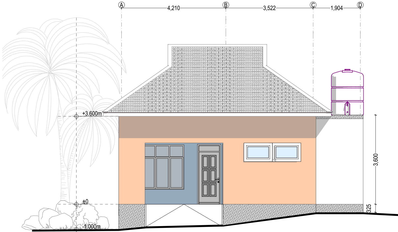
ELEVATION - 01 SCALE 1:75
