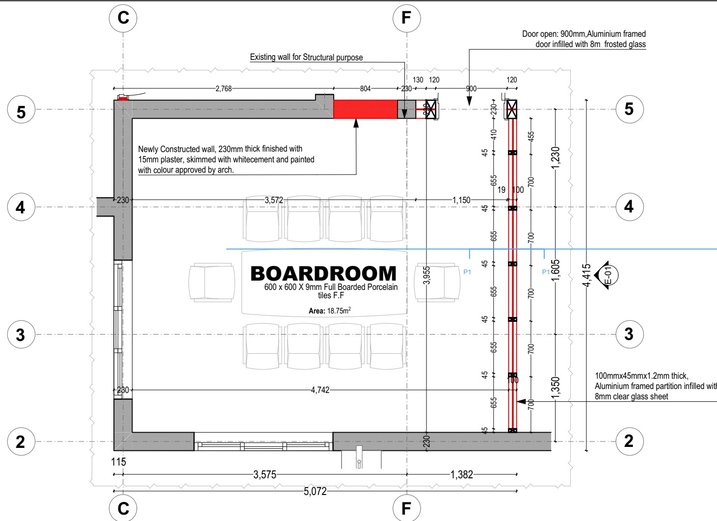
BOARDROOM PARTPLAN + DRY WALL DETAIL SCALE 1:46.73
