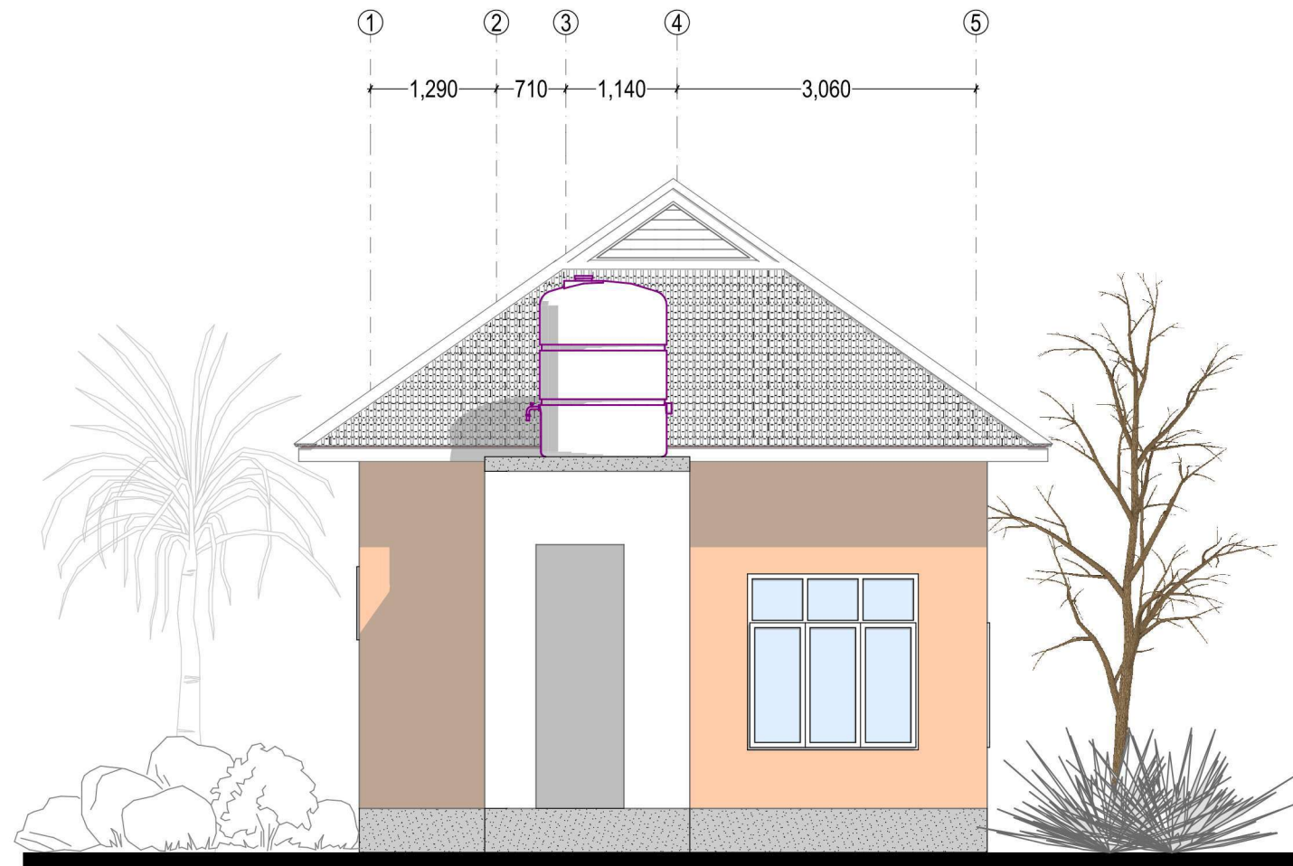
ELEVATION - 03 SCALE 1:70
