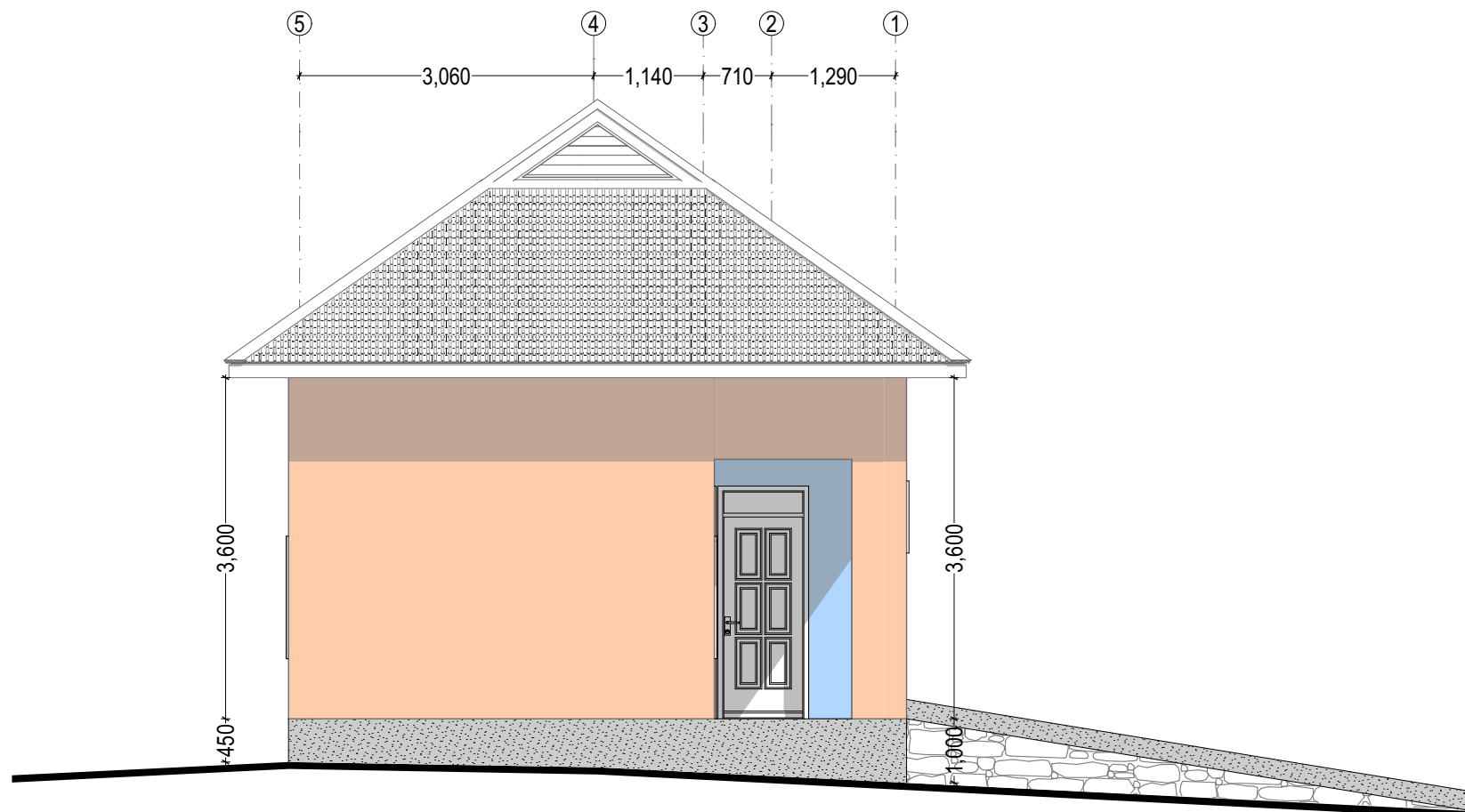
ELEVATION - 0 4 SCALE 1 : 7 0
