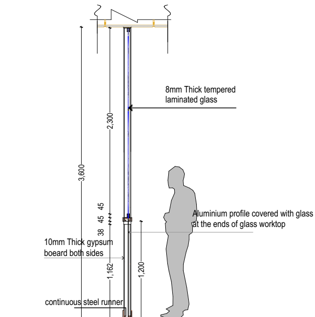
DRY WALL PARTITION DETAILED SECTION SCALE 1:46.73
