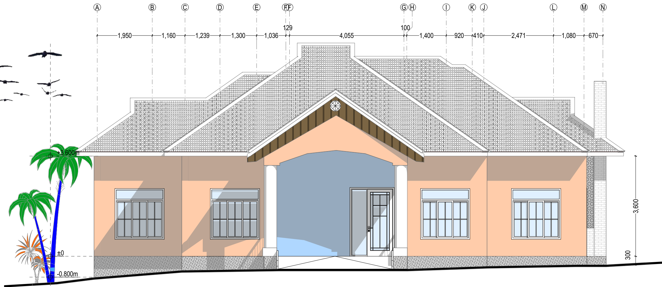
ELEVATION - 01 SCALE 1:80
