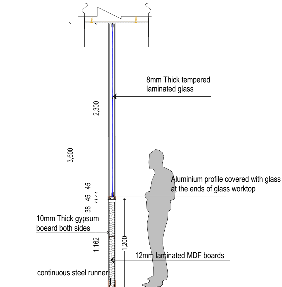
DRY WALL PARTITION DETAILED SECTION SCALE 1:30
