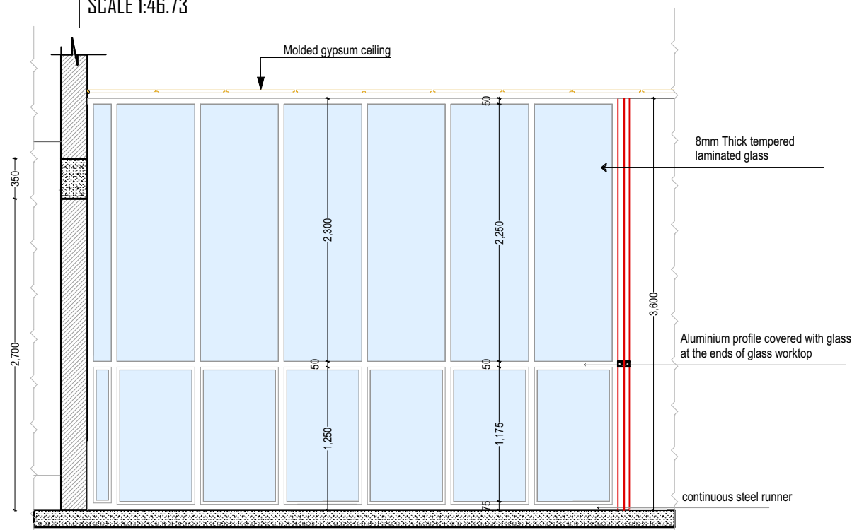
DRY WALL PARTITION DETAILED ELEVATION SCALE 1:46.73
