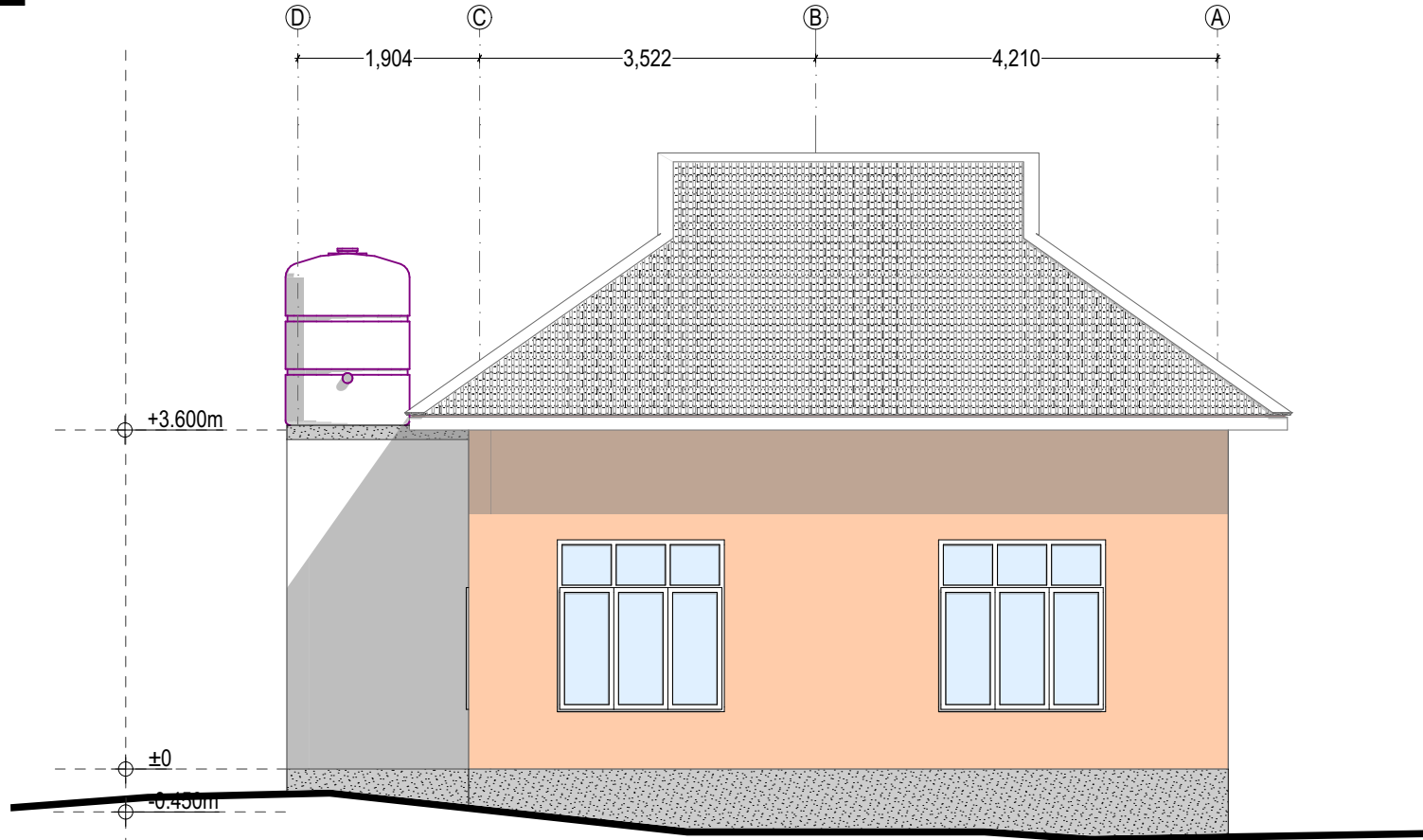
ELEVATION - 02 SCALE 1:75
